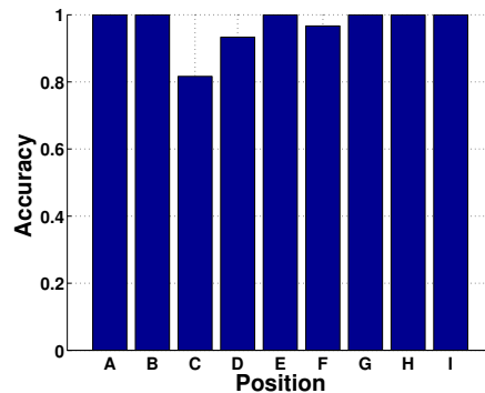
Figure 7: Accuracy of detecting driver phone use at each position in Car I (i.e., positions plotted in Figure 6) under calibrated thresholds with four-channel stereo system.
